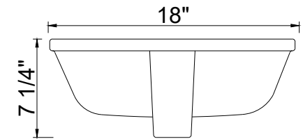
84022 & 84023 DRAWING
